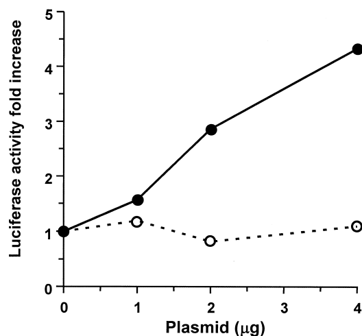
Fig. 5. Dose-response effect of Sp1 and Sp3 on luciferase reporter activity in SL2 cells. SL2 cells were transfected with 0.5 \mu g of pXLO-7-1 and 0.5 \mu g of CMV- \beta -gal with various amounts of CMV-Sp1 (close circles) or CMV-Sp3 (open circles) by calcium phosphate method. The total amount of DNA added was maintained at 5 \mu g with pBSSK. Cells were harvested 48 h after transfection. The expression of luciferase and \beta -galactosidase activity of cell lysate was determined and normalized. The results shown represent the mean of three determinations.
